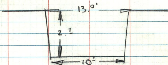
X-SECTION CANAL CROSSING PROPOSED ROAD CHANGE
